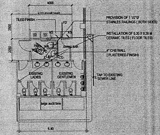
PLUMBING LAYOUT SCALE 1/8" = 1'-0"
