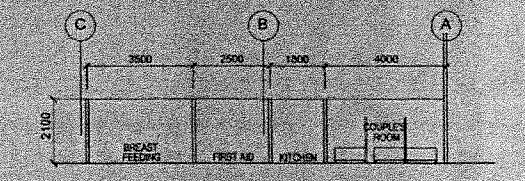
SECTION THRU - B SCALE 1:100 MTS.
