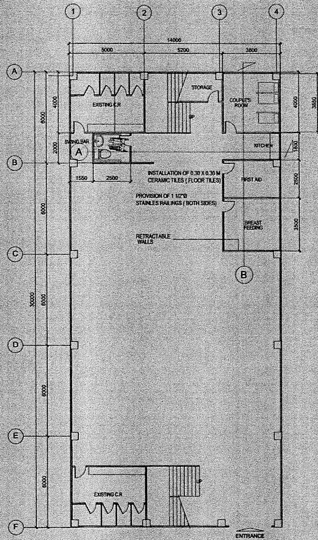
NAGPAYONG MULTI PURPOSE GROUND FLOOR SCALE 1:100 MTS.
